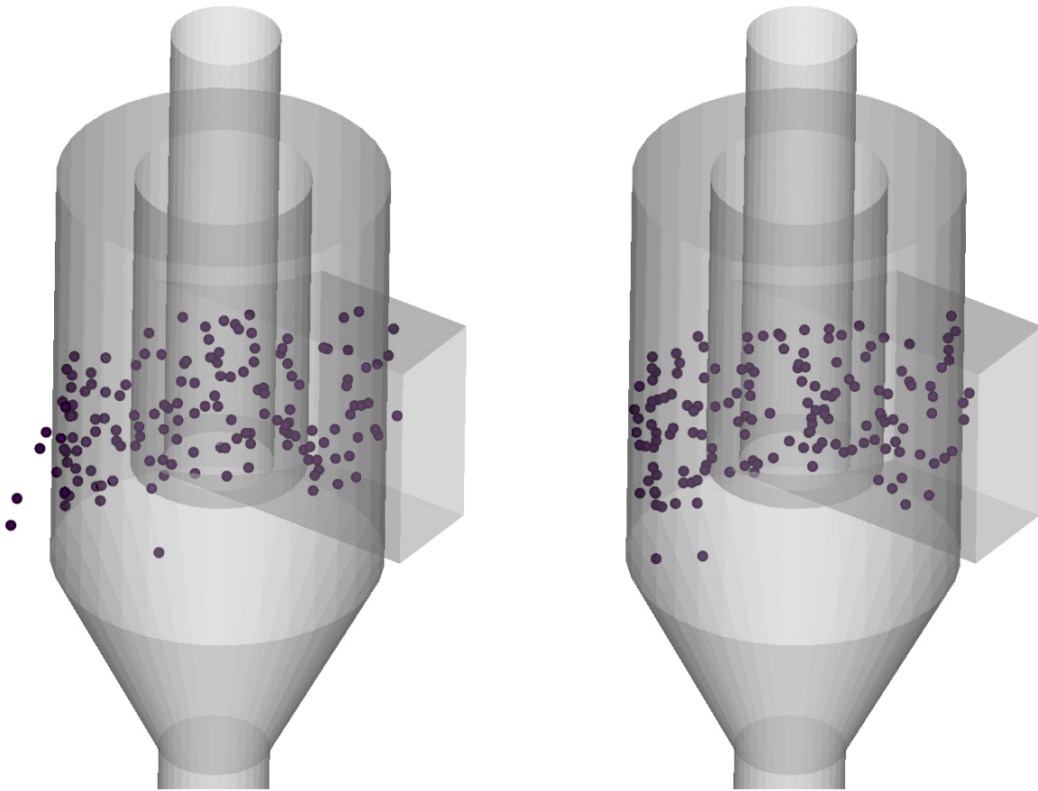
Fig. 8.8: Left: Soft particles ( kn=kn_w=100 N/m) going through the cyclone wall. Right: Harder particles ( kn=kn_w=1000 N/m) bouncing off the wall.
