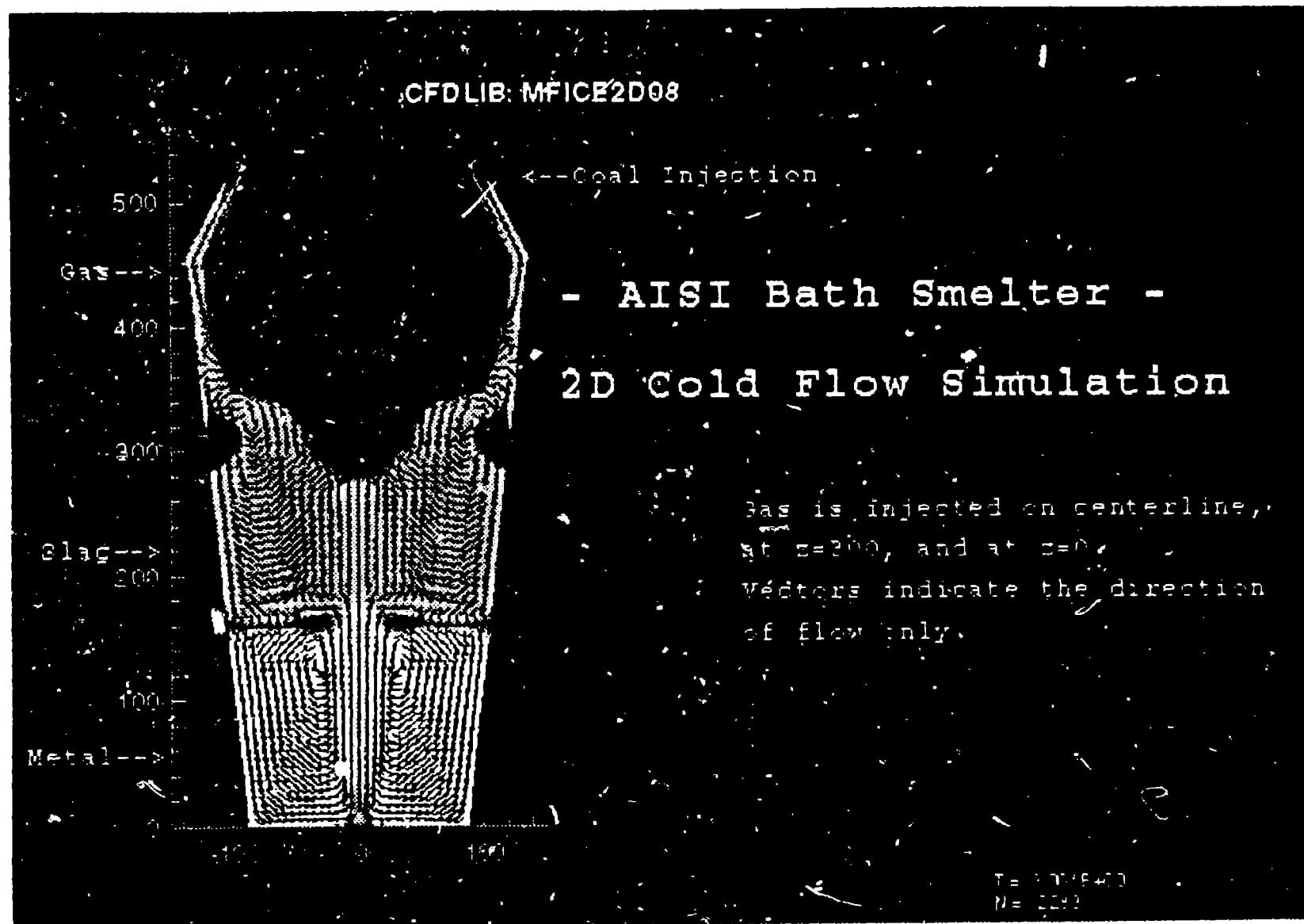
Figure 2 - Bath smelter
