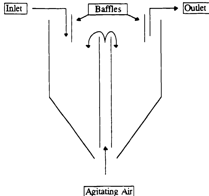
Figure 5 - Schematic Drawing of an Air-Agitated Alumina Crystallizer
