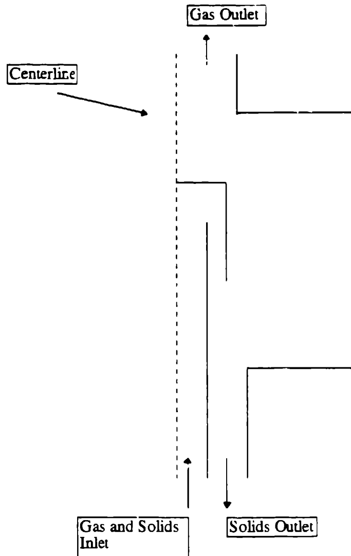
Figure 4 - FCC Riser Separator - Chevron Prototype Multiphase Flow Problem
